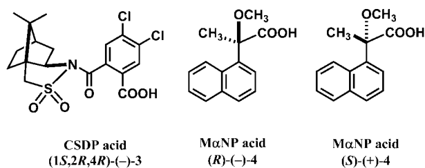
Figure 3. Chiral molecular tools 3 and 4 , useful for enantioresolution of alcohols and determination of their absolute configurations.
