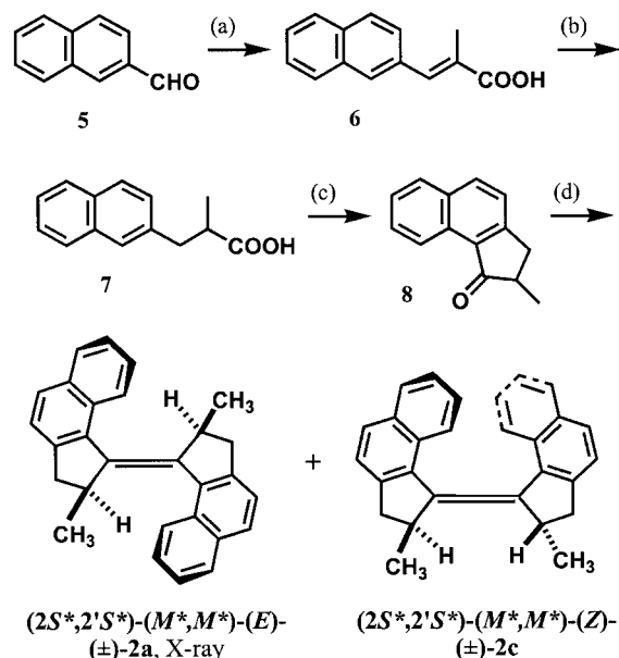
Scheme 1. Synthesis of racemic molecular motor 2 . a) (EtCO) 2 O, EtCOONa, 180 °C, 83%. b) H 2 /Pd-C, EtOH, 87%. c) i) PCl 5 , toluene. ii) SnCl 4 , toluene, 98%. d) TiCl 3 , LiAlH 4 /THF, 80 °C, 96 h, ( E )- 2a , 14% and ( Z )- 2c , 6%.
