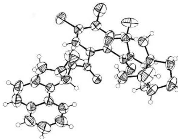
Figure 5. ORTEP drawing of the CSDP ester of cis alcohol ( 1S,2S )-(-)- 11b . The atoms are drawn as 50% probability ellipsoids.
