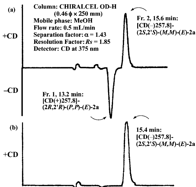
Figure 6. a) Enantioseparation of racemic molecular motor (E)- 2a by chiral HPLC. b) HPLC check of the enantiopurity of synthetic chiral molecular motor [CD(-)257.8]-(2 S ,2' S )-(M,M)-(E)- 2a .
