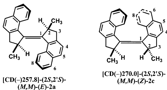
Figure 2. The new light-powered chiral molecular motor of the five-membered ring type and motor rotational isomers, the absolute stereostructures of which were unambiguously determined as shown; the absolute configurational assignment by Feringa's group needs to be revised.
