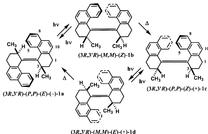
Figure 1. The first light-powered chiral molecular motor of the six-membered ring type, developed jointly by Feringa's group and by our own group, in which the rotational direction of the motor is controlled by the chirality of the molecule.
