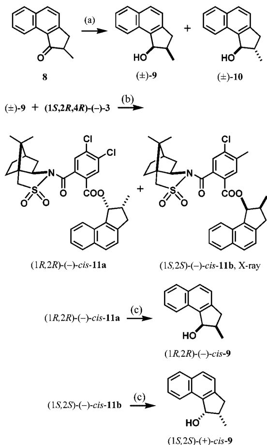
Scheme 2. Preparation of enantiopure cis alcohol 9 by the CSDP acid method. a) \text{LiAlH}_4/\text{THF} , r.t., 9 , 47% and 10 , 51%. b) DCC, DMAP/ \text{CH}_2\text{Cl}_2 , r.t., 11a , 50% and 11b , 49%. c) KOH, \text{CH}_3\text{OH} , 94–96%.
