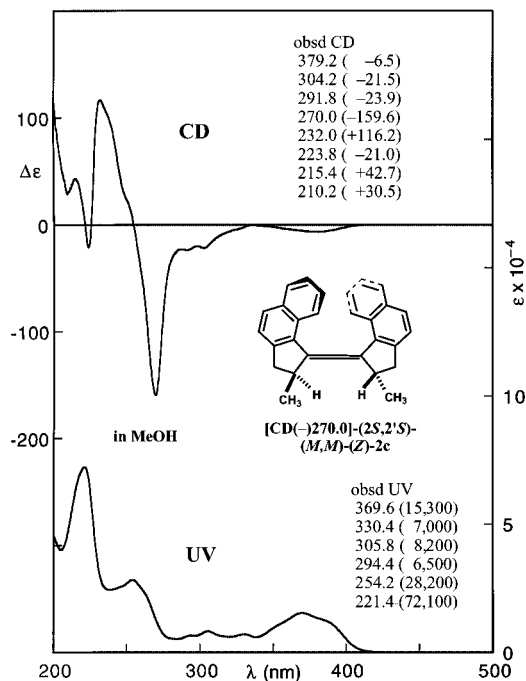
Figure 8. CD and UV spectra of chiral molecular motor [CD(-)270.0]-(2 S ,2' S )-(M,M)-(Z)- 2c in MeOH.
