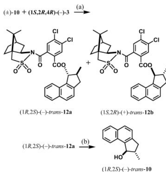
Scheme 3. Preparation of enantiopure trans alcohol 10 by the CSDP acid method. a) DCC, DMAP/ \text{CH}_2\text{Cl}_2 , r.t., 12a , 49% and 12b , 50%. b) KOH, \text{CH}_3\text{OH} , 99%.
