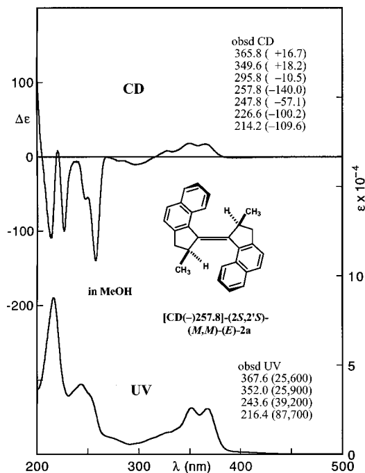
Figure 7. CD and UV spectra of chiral molecular motor [CD(-)257.8]-(2 S ,2' S )-(M,M)-(E)- 2a in MeOH.
