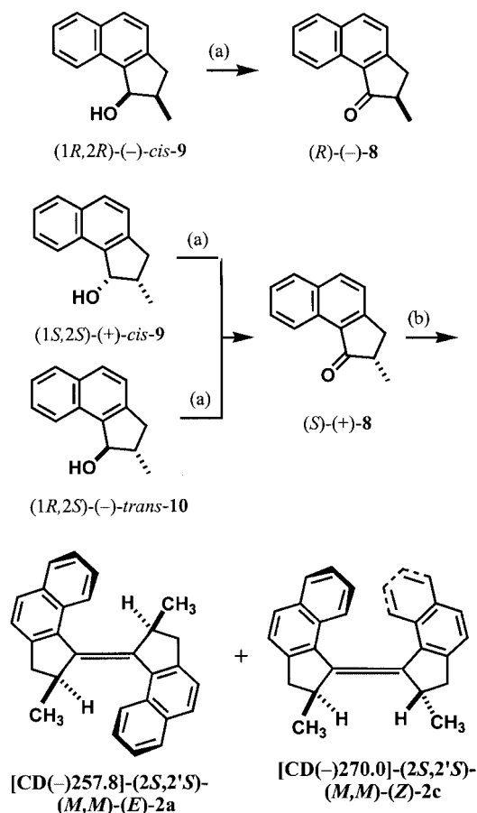
Scheme 4. Synthesis of enantiopure molecular motor 2 . (a) PCC, MS 4 A, CH 2 Cl 2 , 88–96%. (b) TiCl 3 , LiAlH 4 /THF, reflux, 4 h, [CD(–)257.8]-(E)- 2a , 21% and [CD(–)270.0]-(Z)- 2c , 5%.
