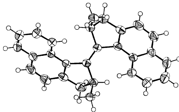
Figure 4. ORTEP drawing of trans -olefin ( \pm )- 2a . The atoms are drawn as 50% probability ellipsoids.
